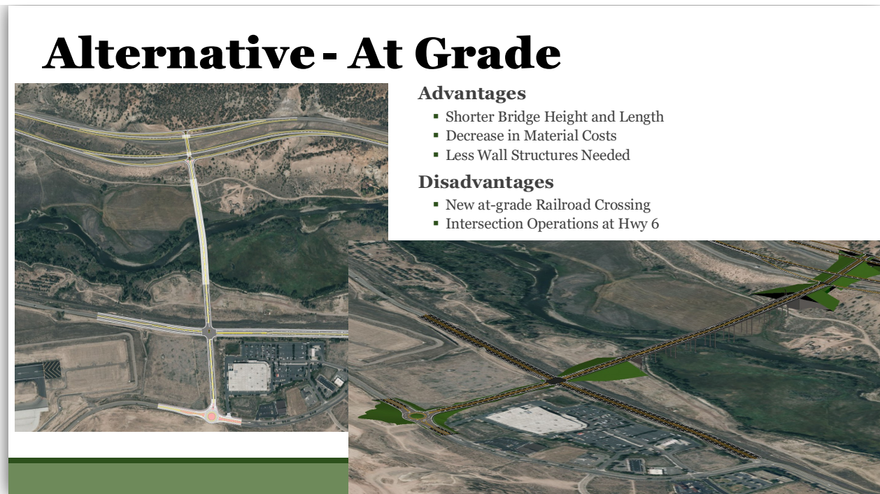
Figure 9 – Alternative – At-Grade
